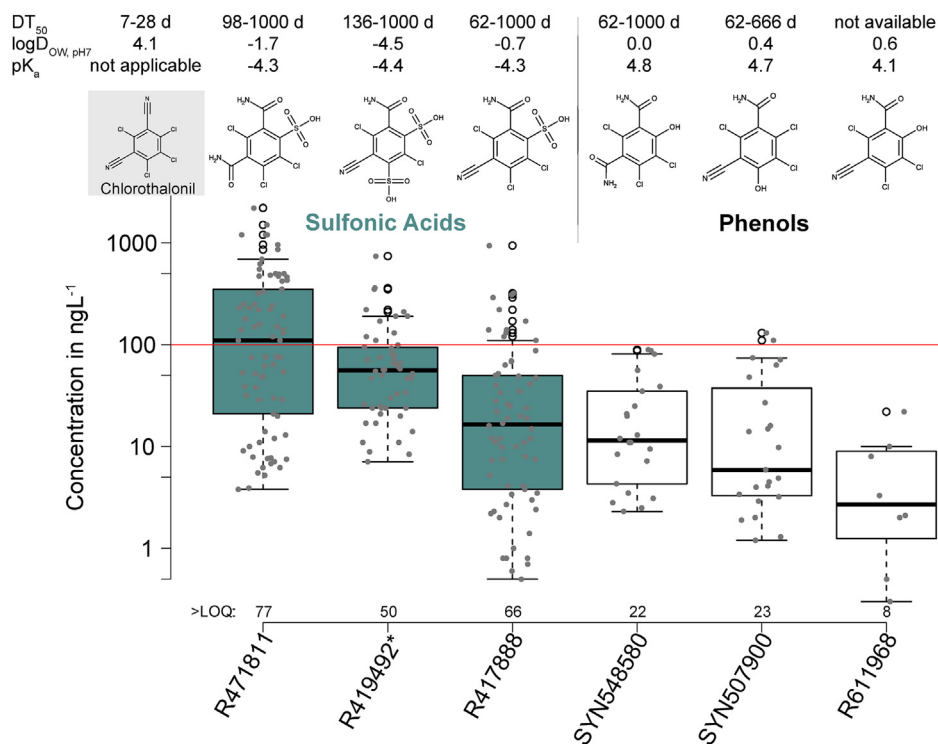
Fig. 1. Concentration distribution of different chlorothalonil TPs in 77 samples (73 x groundwater, 4 x surface water). Non-detects (LOQs: 0.2–5 ng L -1 ) are not included in the boxplots. The sulfonic acid-containing TPs (on the left in green) were more frequently detected and at higher concentrations than the phenol-containing TPs (on the right in white). The red line marks the Swiss drinking water standard. The open circles represent outliers. The gray solid circles show the concentrations of individual samples. Dissipation time DT 50 from EFSA (2018), logD OW, pH7 (water-n-octanol distribution coefficient considering the speciation at pH 7) and pK a (acid dissociation constant) were predicted with JChem for Office (Version 17.1.2300.1455; ChemAxon Ltd.). *R419492: high measurement uncertainty (~0.5–2 × reported concentration). (For interpretation of the references to colour in this figure legend, the reader is referred to the Web version of this article.)
